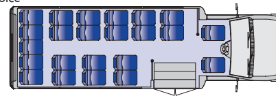
22 passengers and driver
