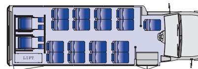
16 passengers plus 2 wheelchairs and driver
